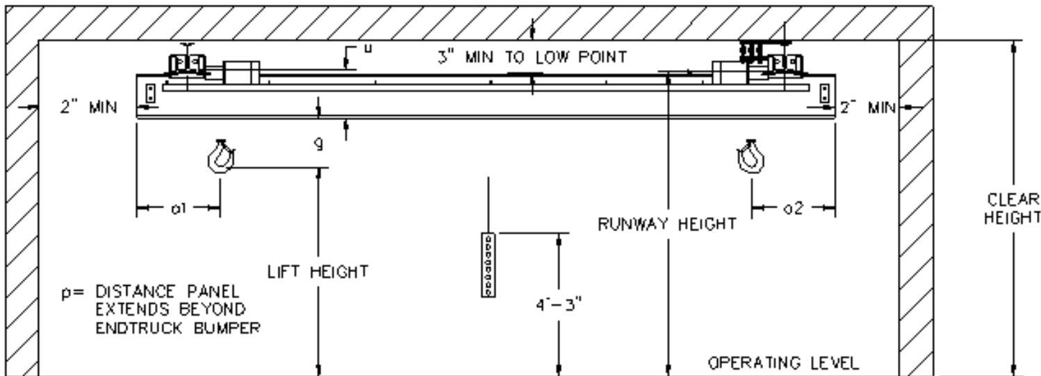
UNDERRUNNING SINGLE GIRDER CRANE
